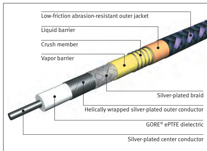
Figure 6: Cable Construction
