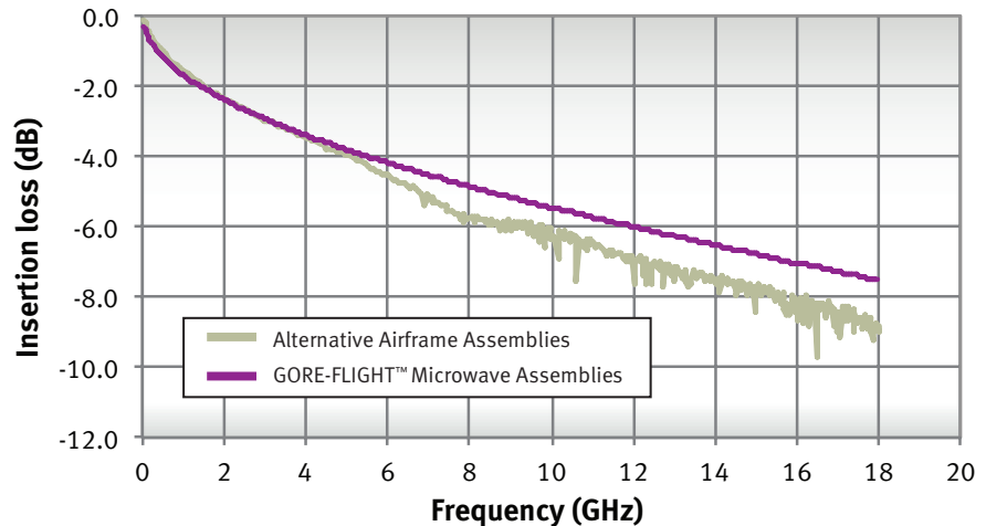
Figure 3: Insertion loss of cable assemblies after installation
